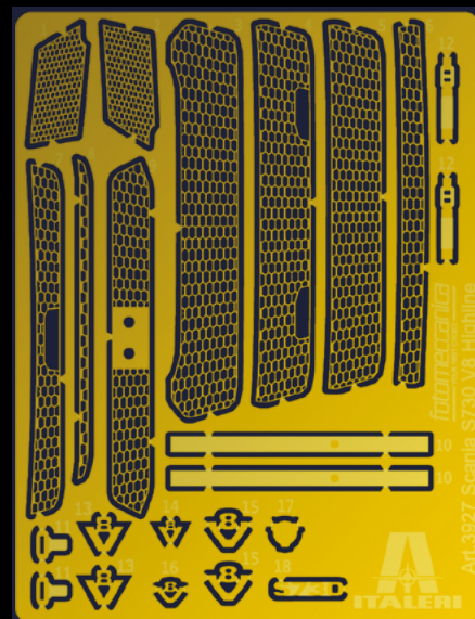
Photo-etched fret
